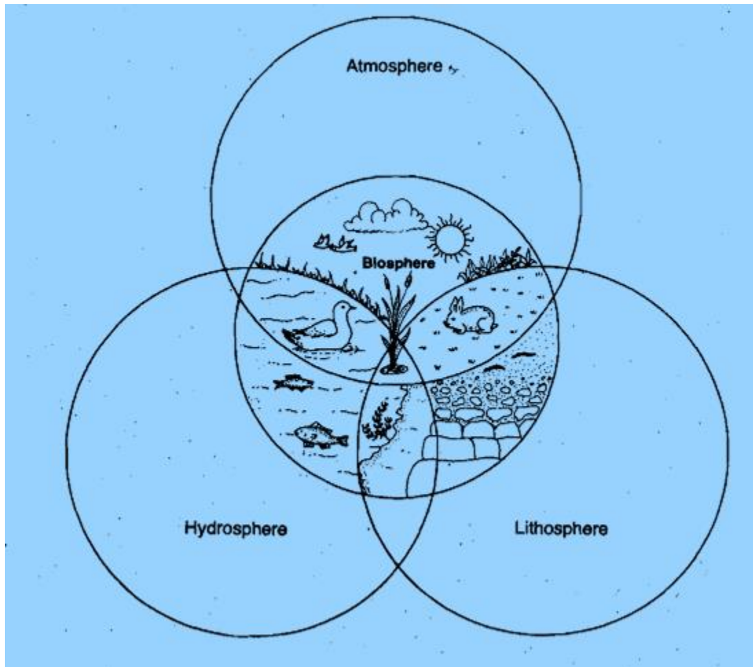
Fig: 1.2 idealised scheme of the biosphere
