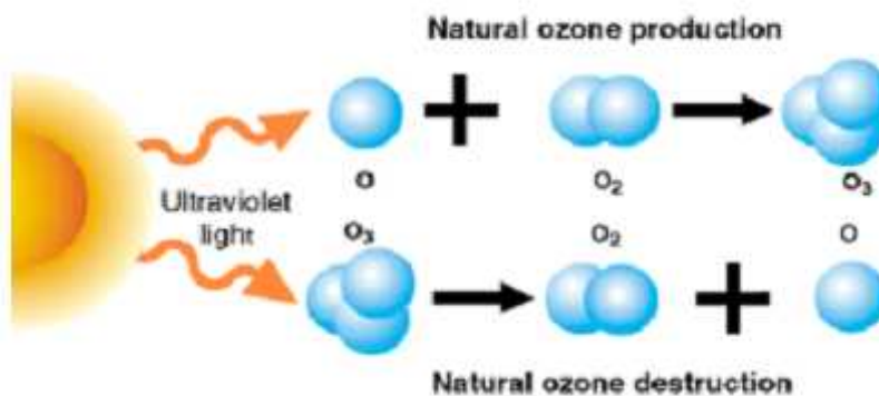
Fig: 2.2 Ozone production and destruction process
