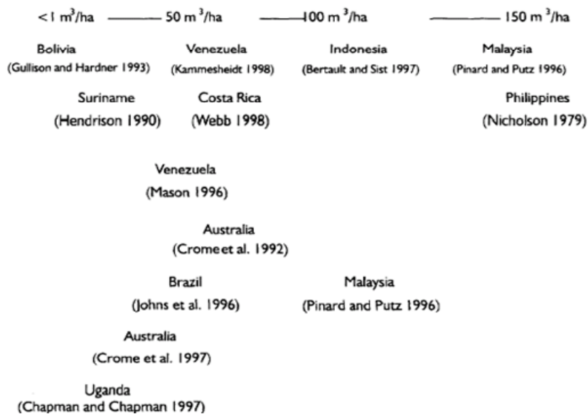
Figure 1 Logging intensities ( \text{m}^3/\text{ha} ) for tropical forests. From Putz et al. 2001
