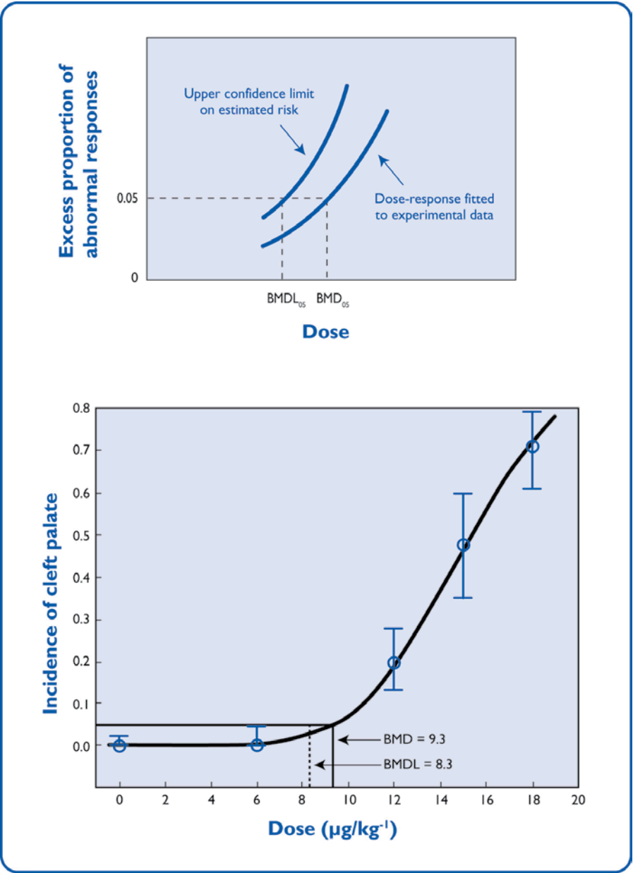
(a) stylised to show the extrapolation of BMD_{05} and its lower confidence limit (based on upper confidence limit of incidence) (b) illustration of BMD calculation from real data on malformations induced by TCDD Sand et al. (2008) using data from Birnbaum et al. (1989)
